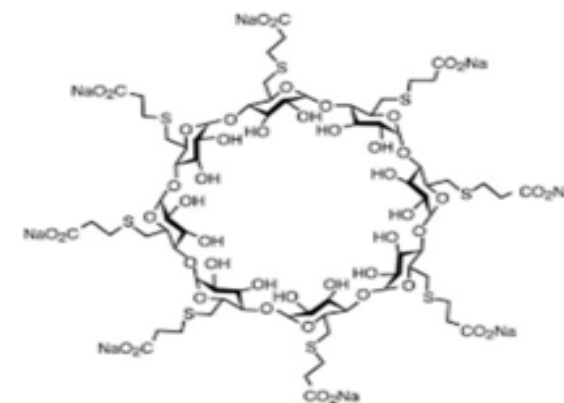
Sugammadex sodium
