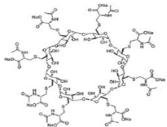
Adamgammadex sodium
